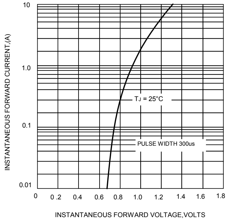
FIG.4-TYPICAL FORWARD CHARACTERISTICS
